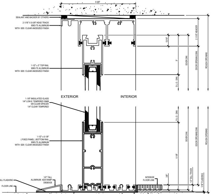
B Section @ (Fixed) Max-Slider Sliding Glass Door (XO) with screen
