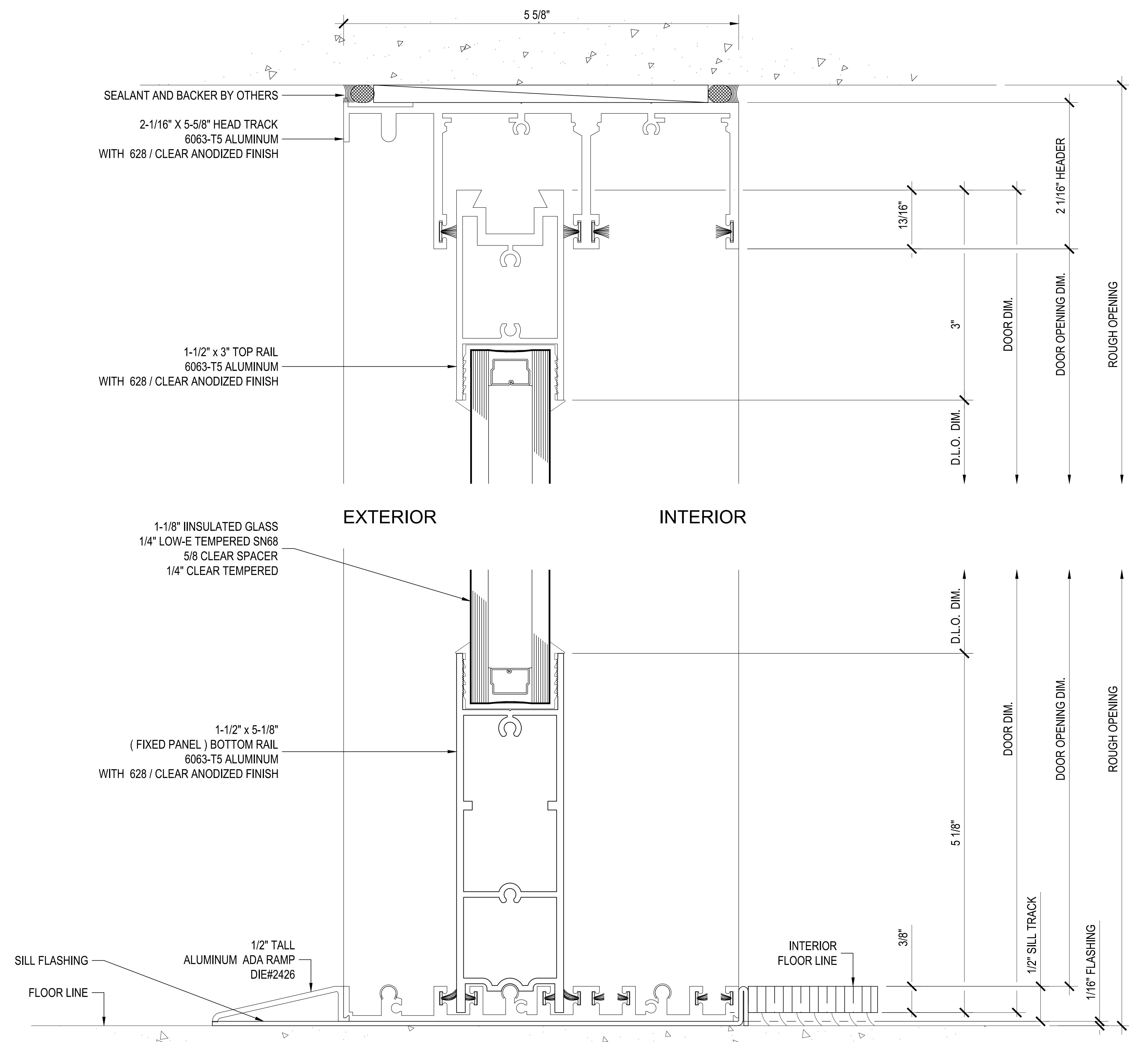
Section @ (Fixed) Max-Slider Sliding Glass Door (XO) with screen
