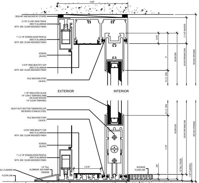
C Section @ (Slider) Max-Slider Sliding Glass Door (XO) with screen
