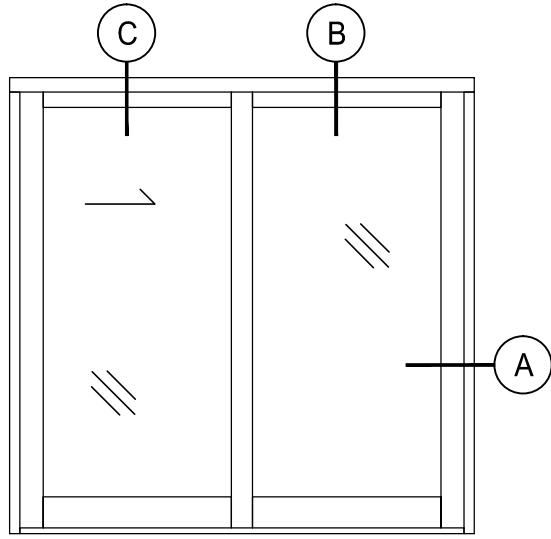
C Section @ (Slider) Max-Slider Sliding Glass Door (XO) with screen
