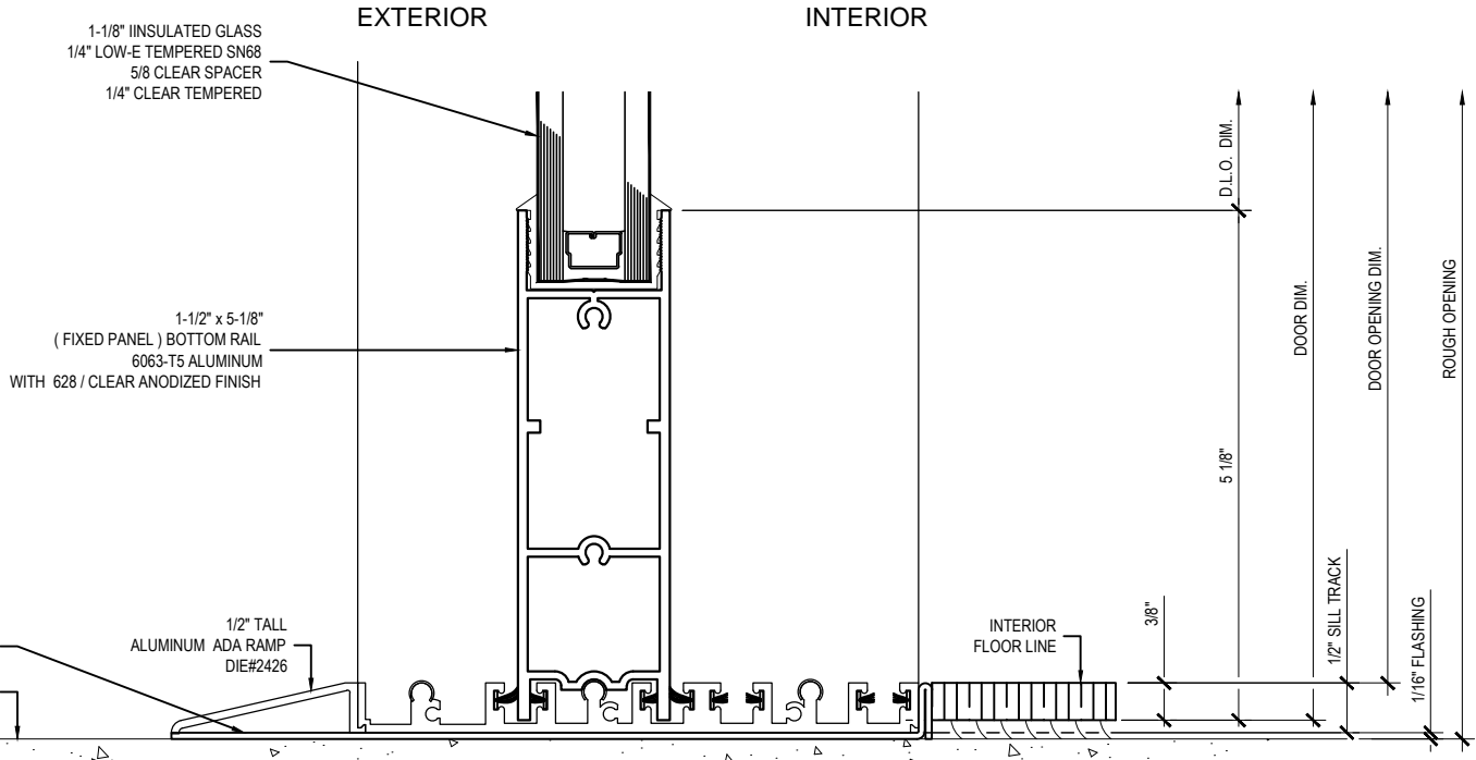
B Section @ (Fixed) Max-Slider Sliding Glass Door (XO) with screen
